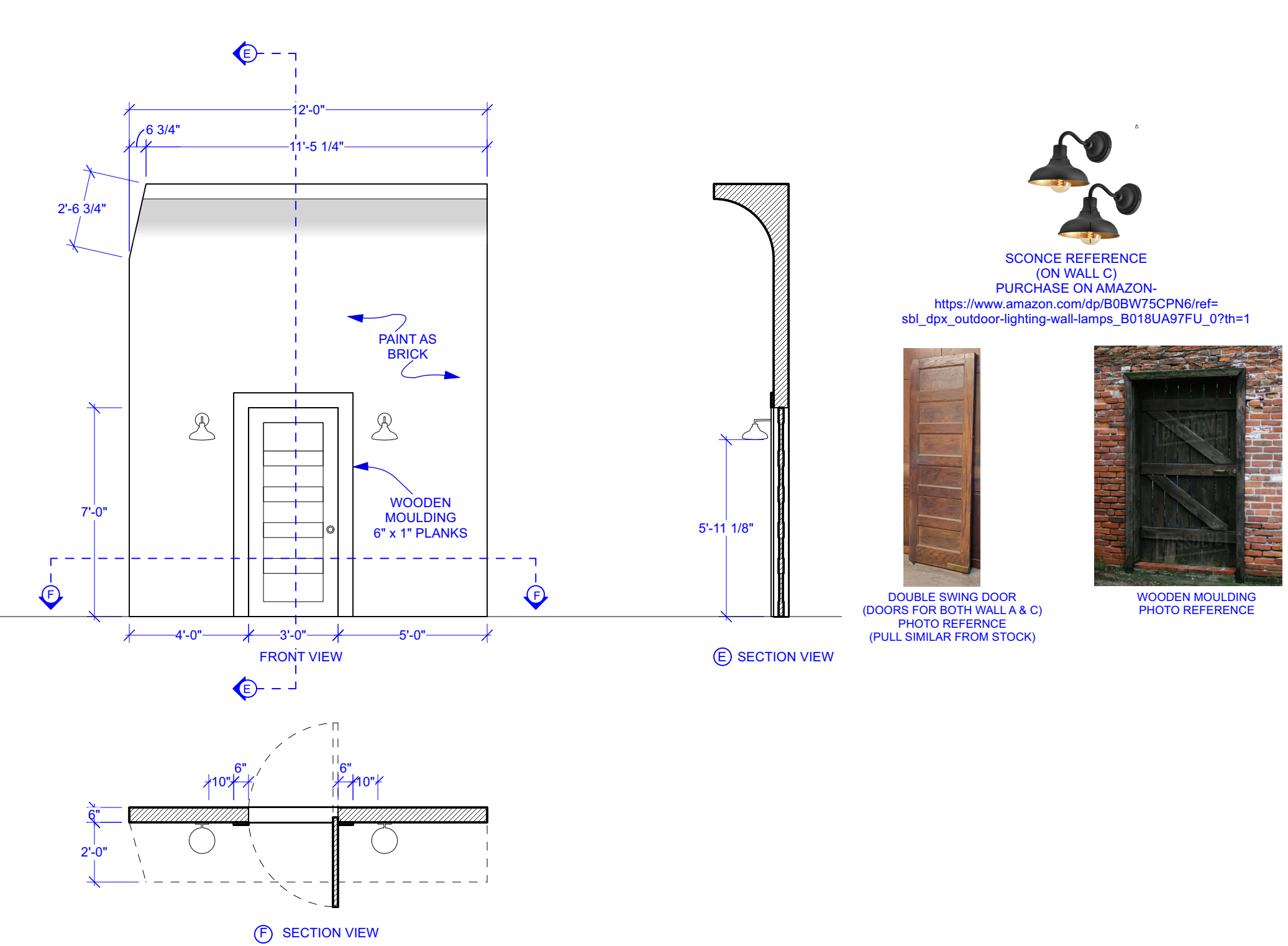
WALL C SCALE : 1/4" = 1'-0"
