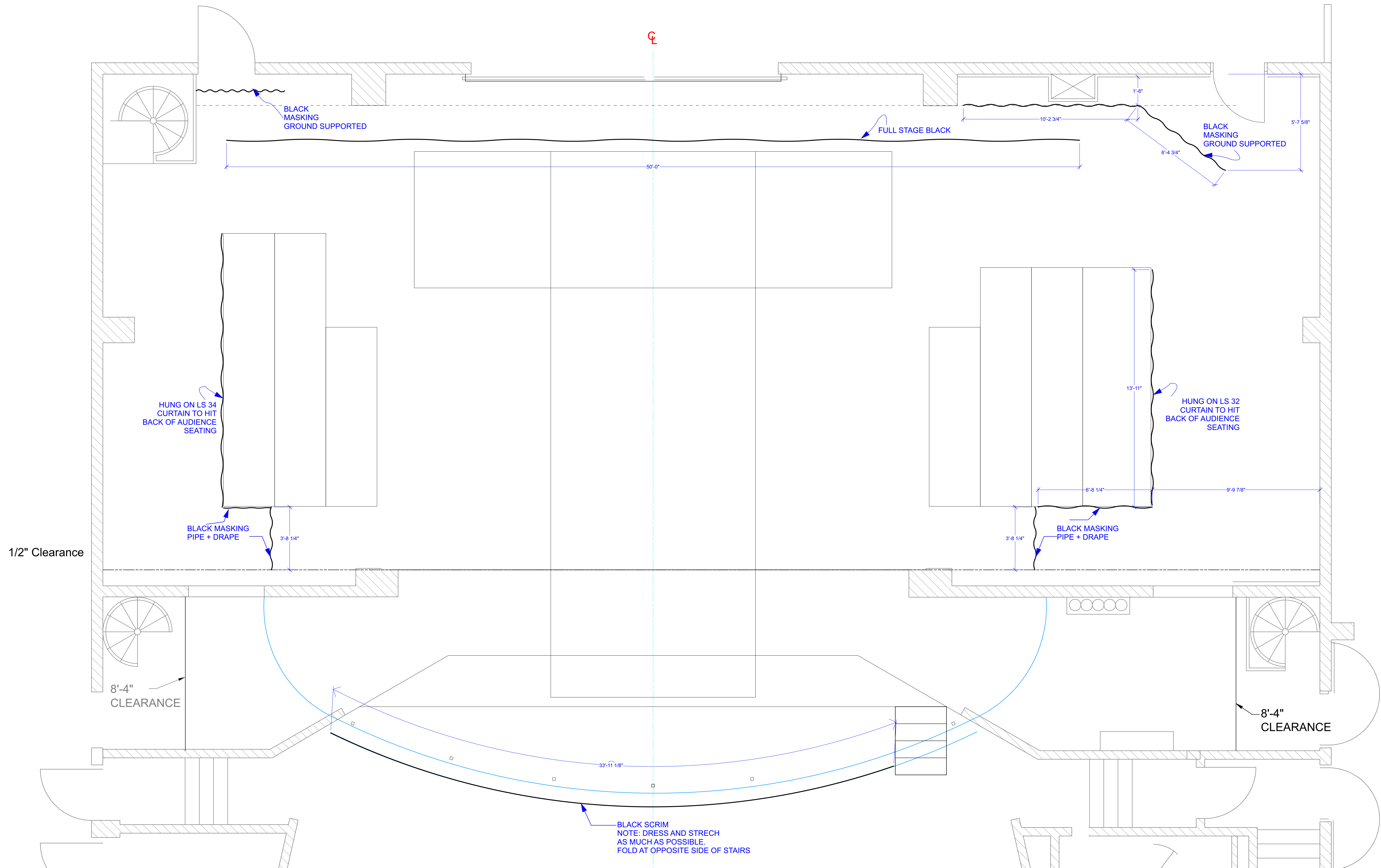
MASKING PLAN SCALE : 3/8" = 1'-0"
