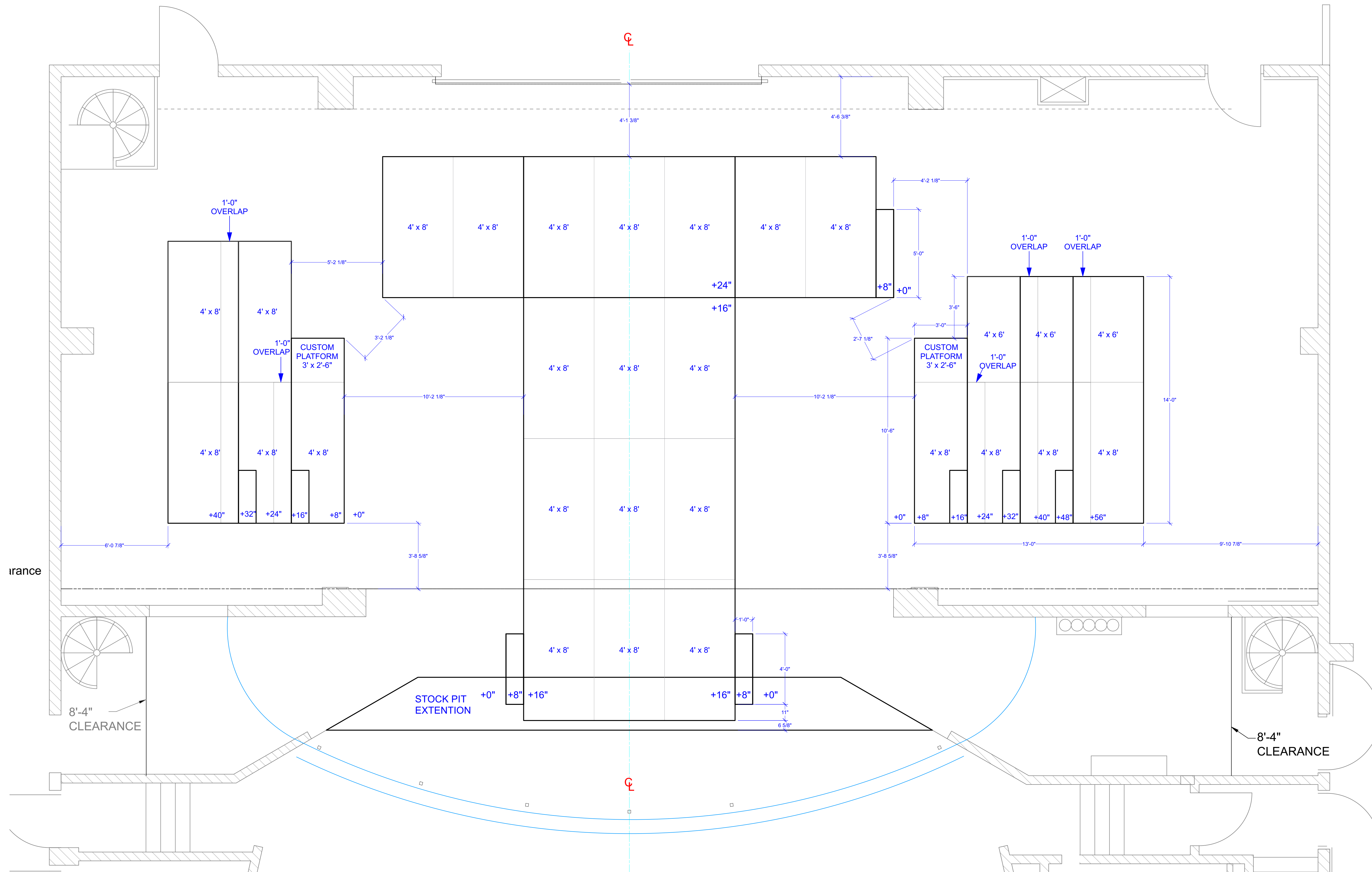
DECK PLAN SCALE : 3/8" = 1'-0"
