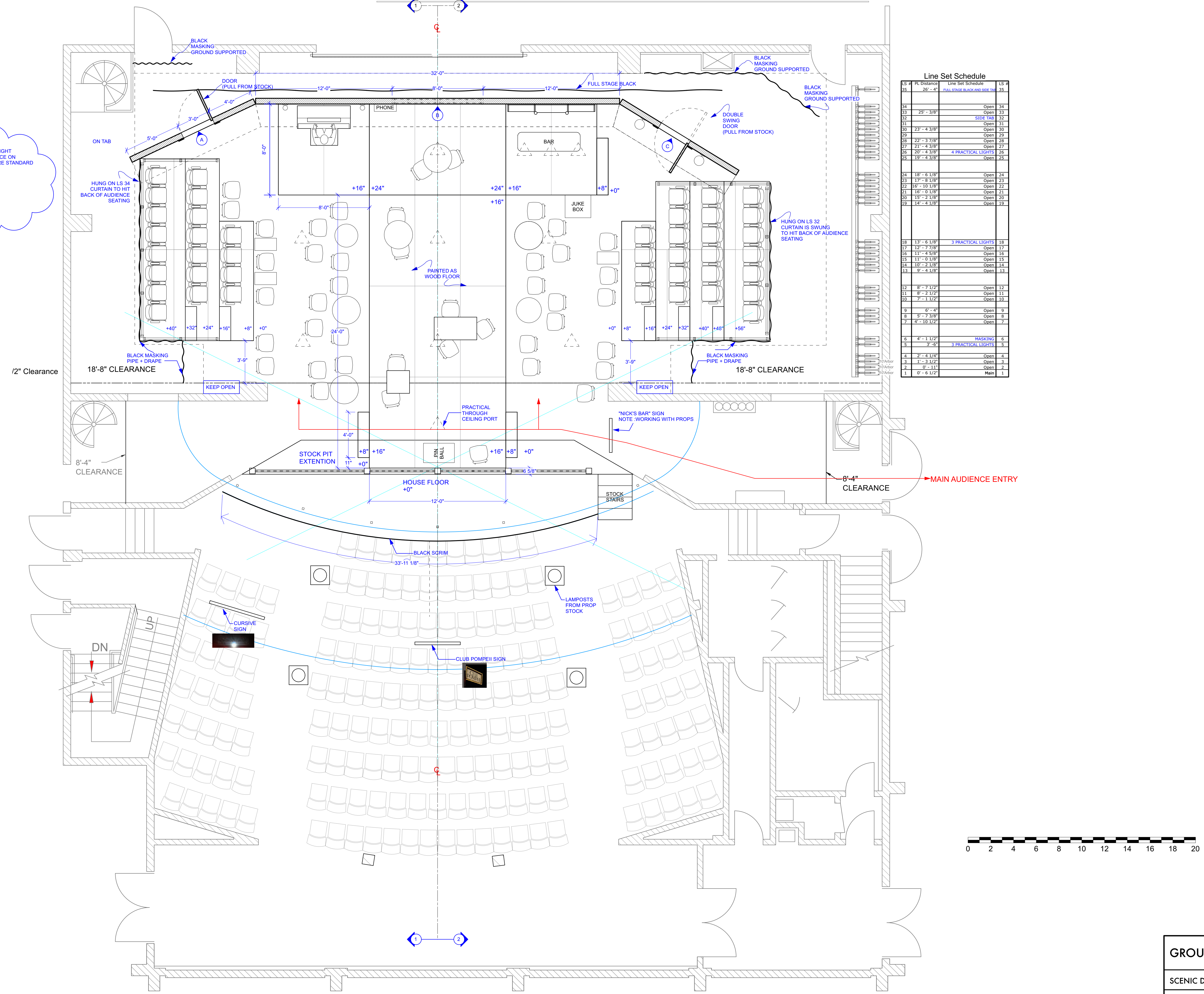
GROUND PLAN SCALE: 1/4" = 1'-0"
