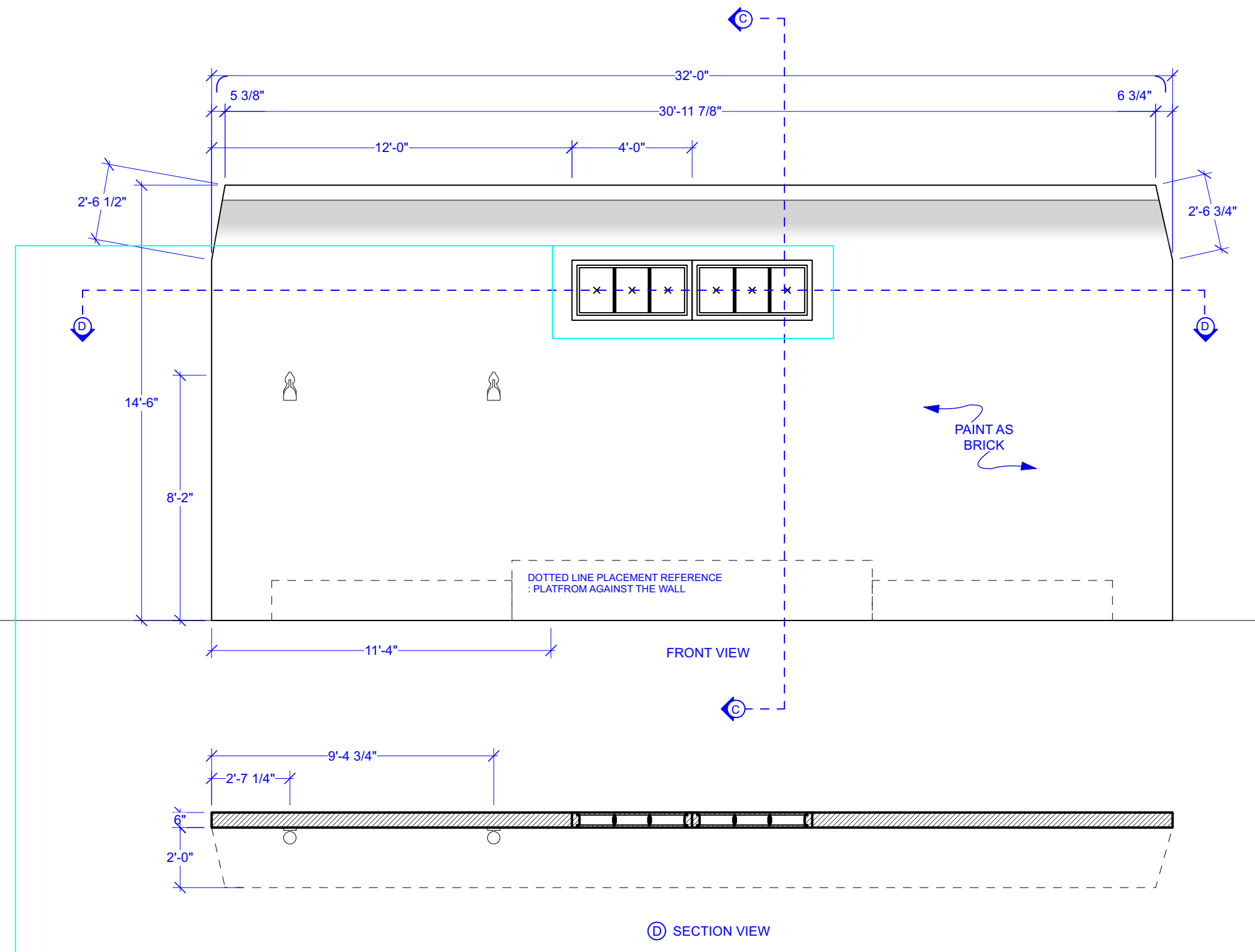
WALL B SCALE : 1/4" = 1'-0"
