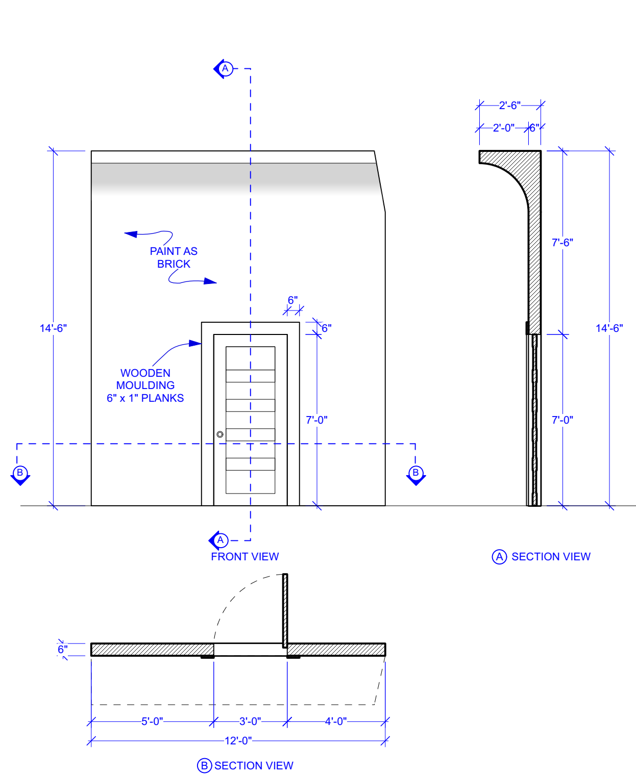
WALL A SCALE : 1/4" = 1'-0"
