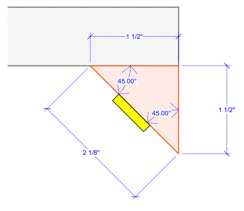
DETAIL: SECTION (H) BLOWUP - TRIANGLE+ LED UNIT SCALE : FULL SCALE
