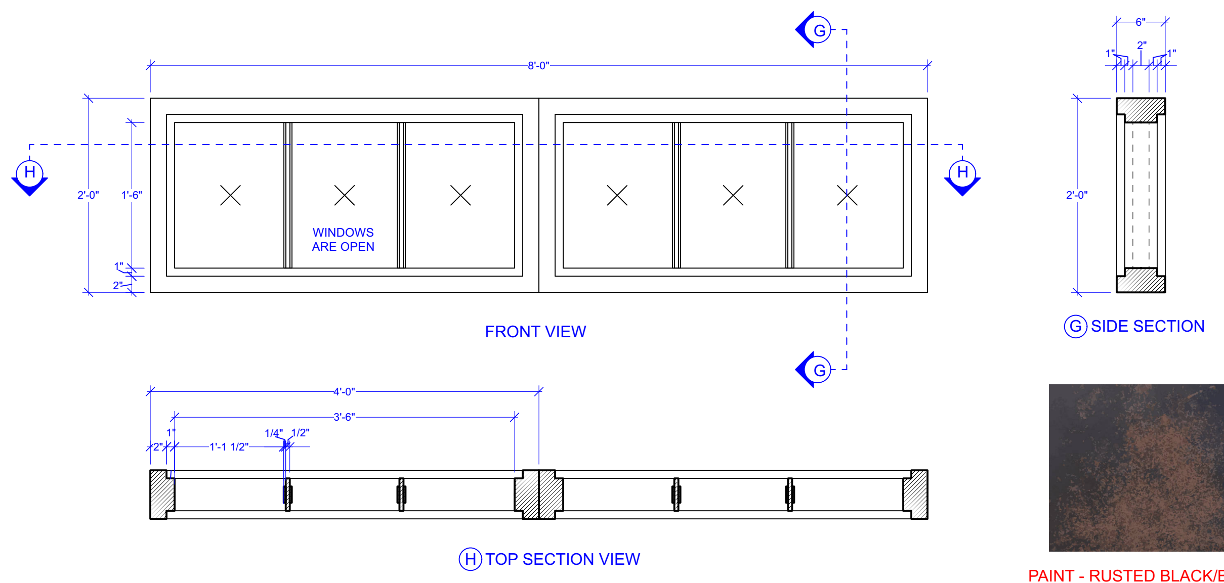
WINDOW DETAIL ON WALL B SCALE : 1" = 1'-0"
